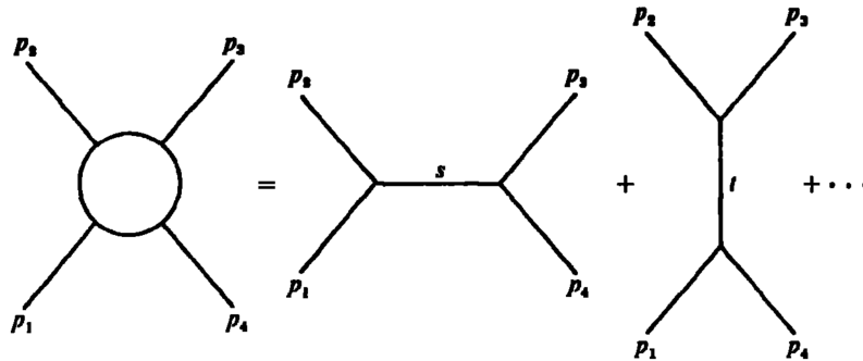
Figure 1.1. An elastic scattering process with incoming particles with momenta p_1, p_2 and outgoing particles with momenta -p_3, -p_4 (we adopt the convention that the labels refer to incoming momenta). Both s - and t -channel diagrams are indicated. In field theory the amplitude is constructed as a sum of s -channel and t -channel diagrams.
